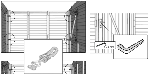
Fasten the tension locks and the door handle
