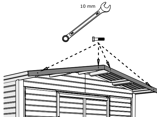
Install the fascia boards
