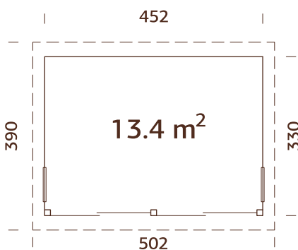
Annabel 13,4 m 2 kit without sliding door
